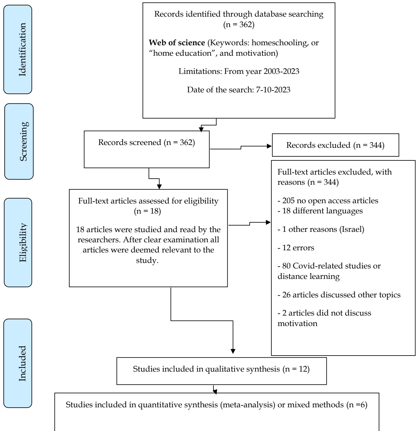
Figure 1: PRISMA Diagram
